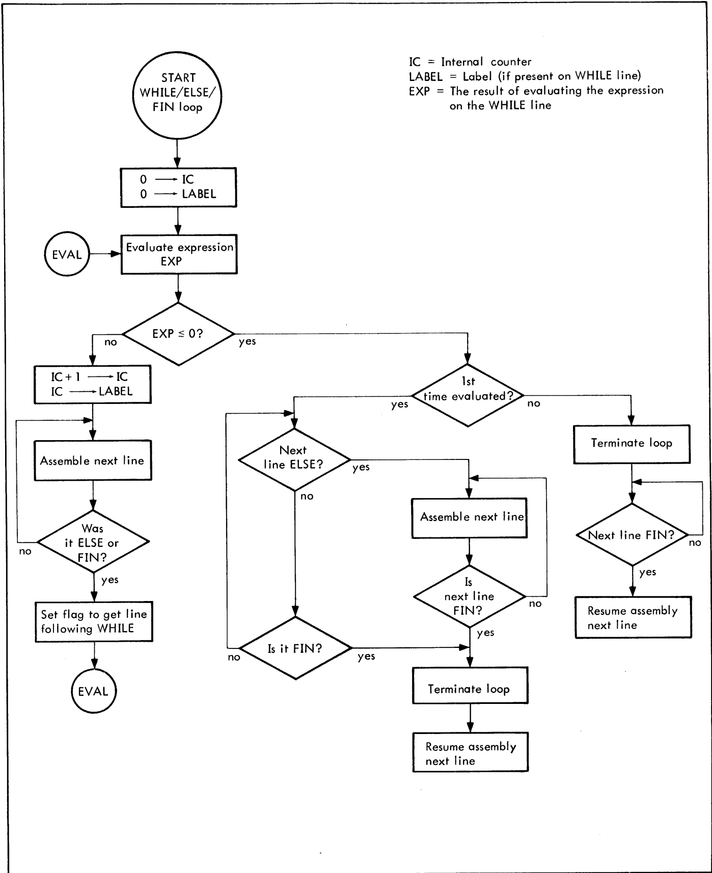
Figure 2. Flowchart of WHILE/ELSE/FIN Loop
