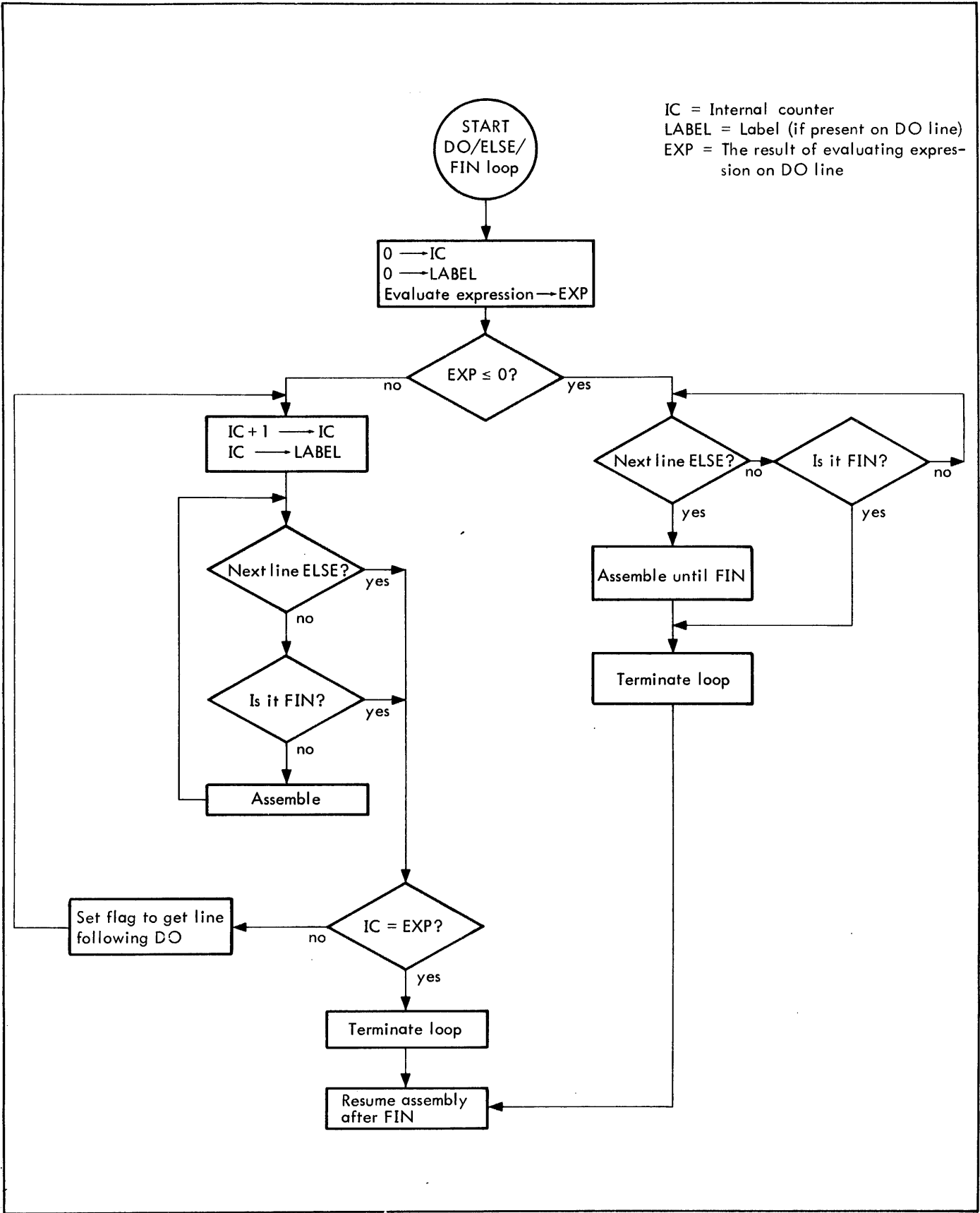
Figure 3. Flowchart of DO/ELSE/FIN Loop
